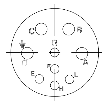
针位排布图 Contact arrangement
