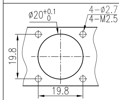
面板安装开孔图 Panel cut out
