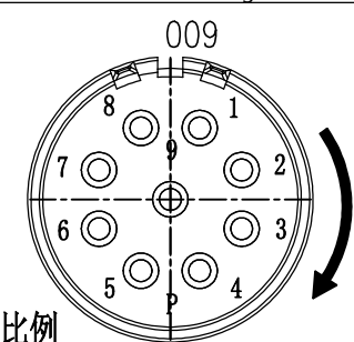
针位排布图 Contact arrangement
