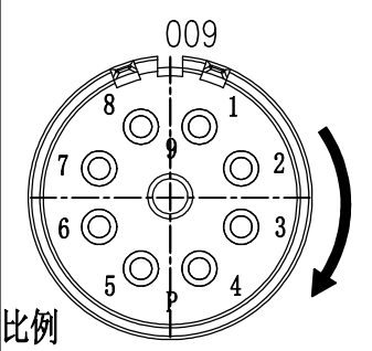
针位排布图 Contact arrangement
