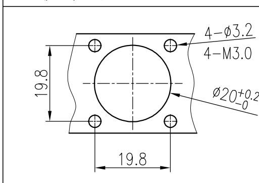
面板安装开孔图 Panel cut out
