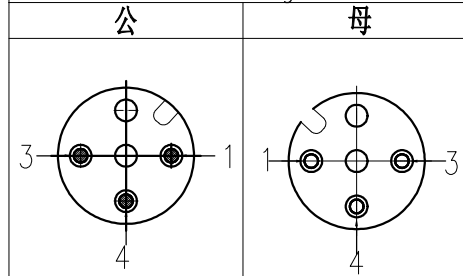
Contact arrangements
