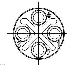
针位排布图 Contact arrangement
