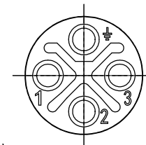
针位排布图 Contact arrangement
