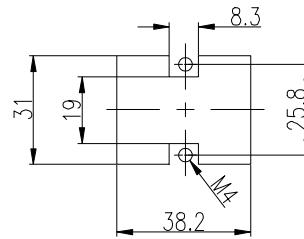
面板开孔图 Panel cut out
