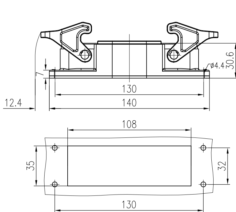
面板开孔图 Panel cut out
