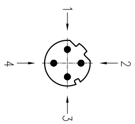
针位图 Contact arrangements
