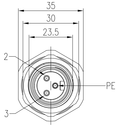
针位排布图 Contact arrangement
